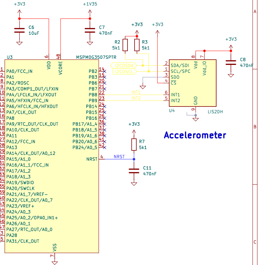
MSPM0 Microcontroller
