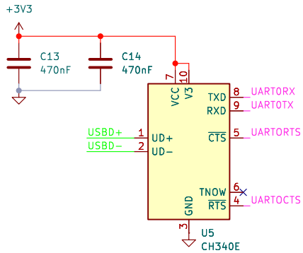
USB-UART Converter
