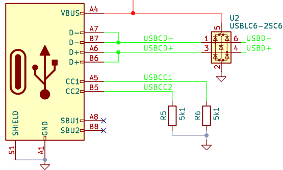
USB-C Connector
