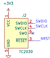
SWD Header
